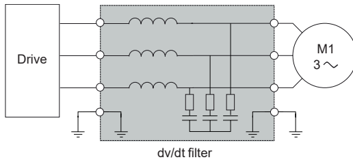
Altivar machine drive with dv/dt filter
